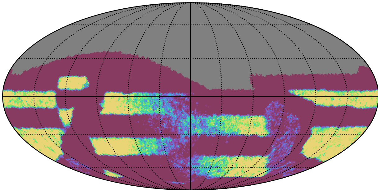
no_high_blob_v3.3_10yrs Yr 3-4 all bands: NVisits
