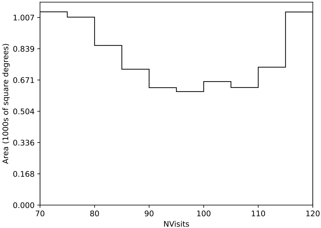
no_high_blob_v3.3_10yrs Yr 3-4 all bands: NVisits
