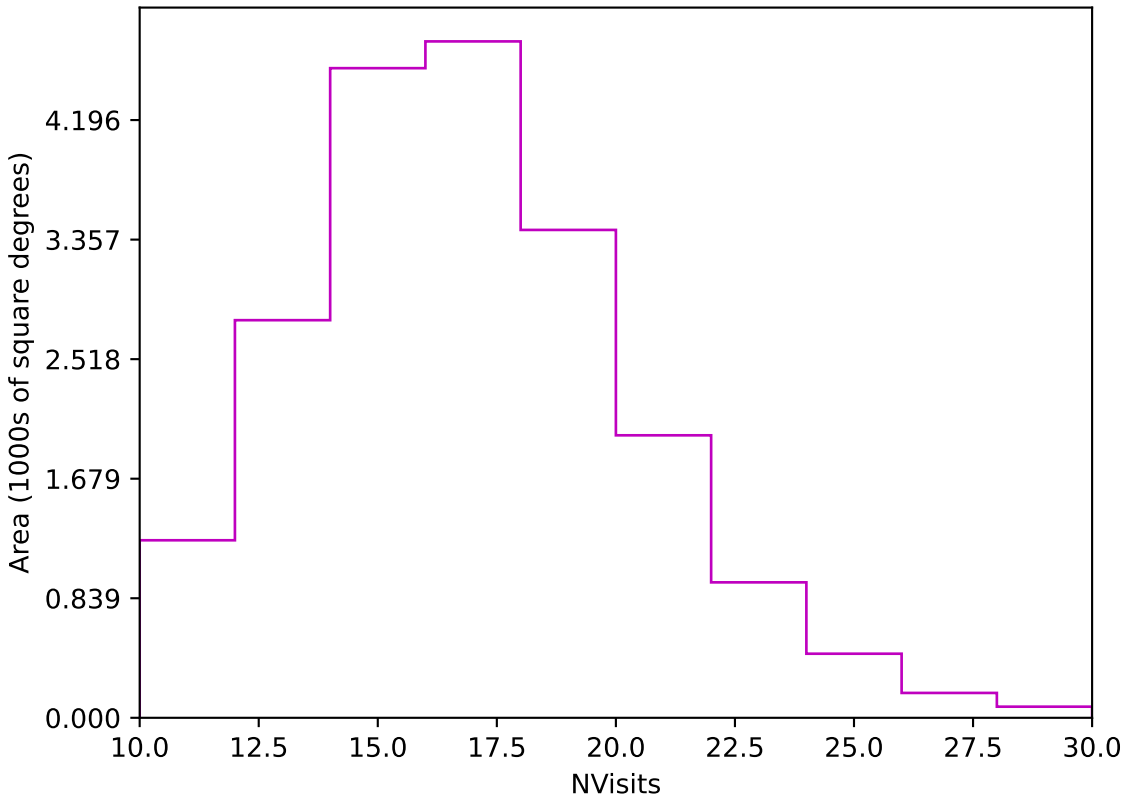
no_high_blob_v3.3_10yrs Yr 1 z band: NVisits
