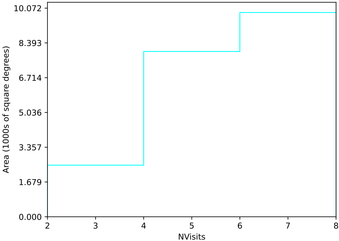
no_high_blob_v3.3_10yrs Yr 1 u band: NVisits
