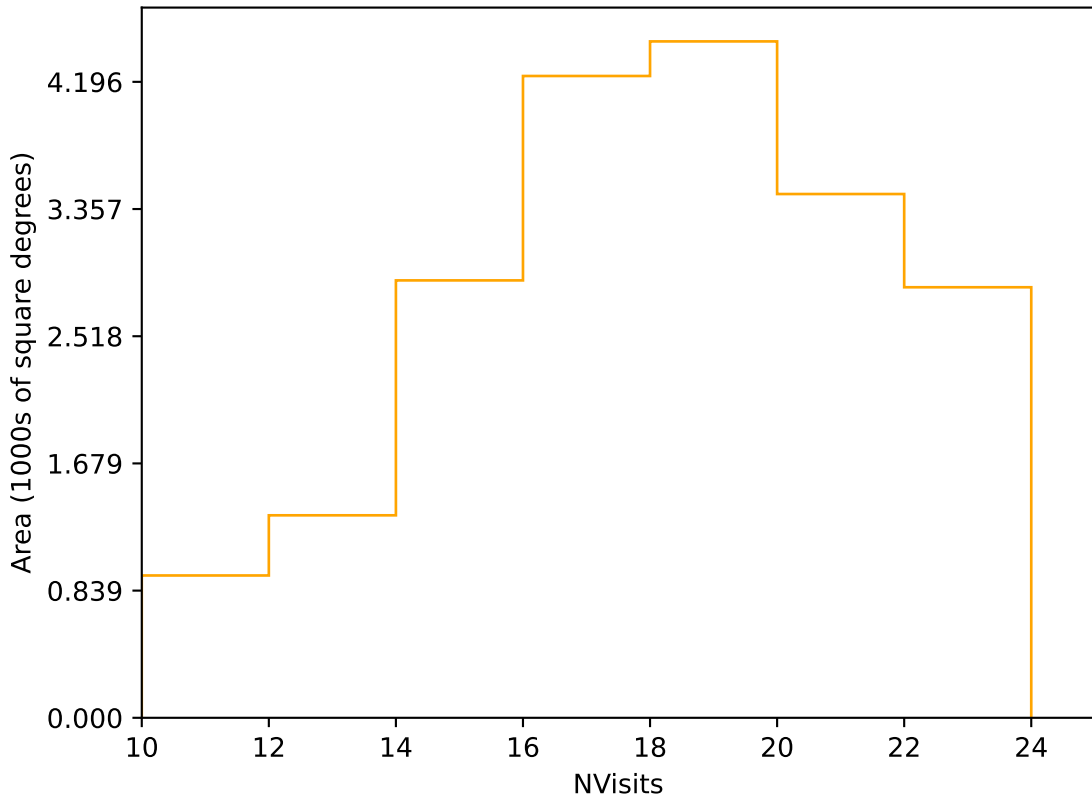
no_high_blob_v3.3_10yrs Yr 1 r band: NVisits
