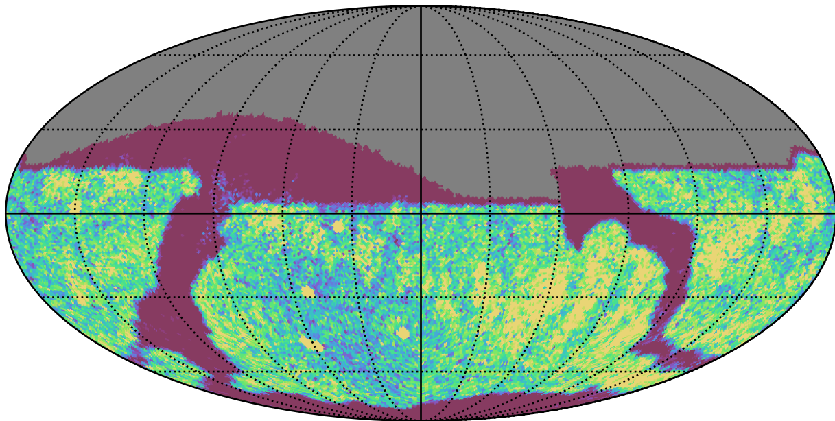
no_high_blob_v3.3_10yrs Yr 1 i band: NVisits
