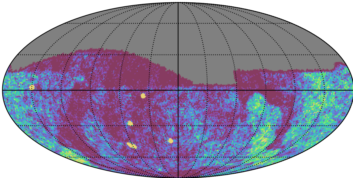
no_high_blob_v3.3_10yrs Yr 1 g band: NVisits
