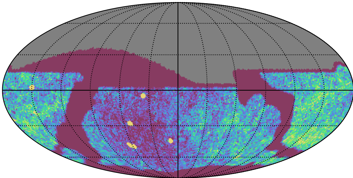
no_high_blob_v3.3_10yrs Yr 1 all bands: NVisits
