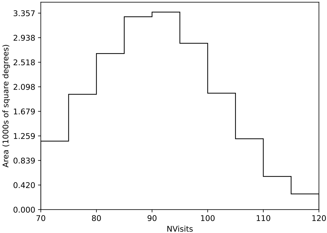
no_high_blob_v3.3_10yrs Yr 1 all bands: NVisits
