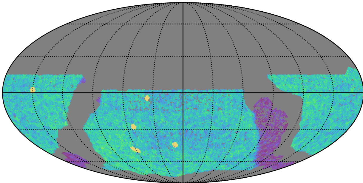
no_high_blob_v3.3_10yrs WFD u band: NVisits
