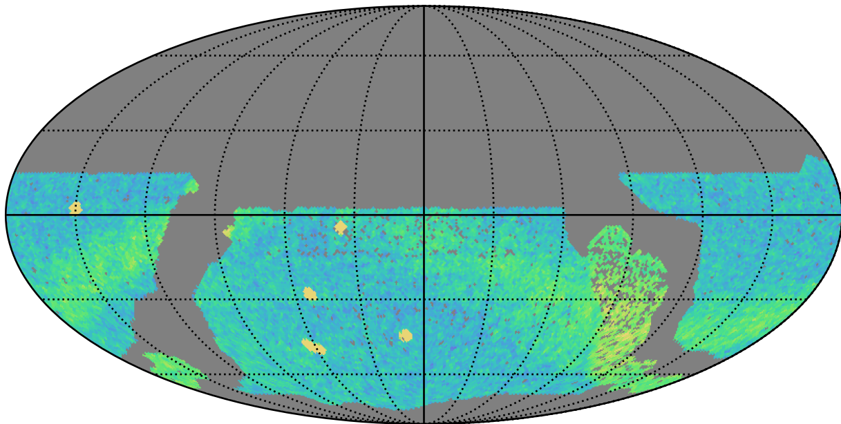
no_high_blob_v3.3_10yrs WFD r band: NVisits
