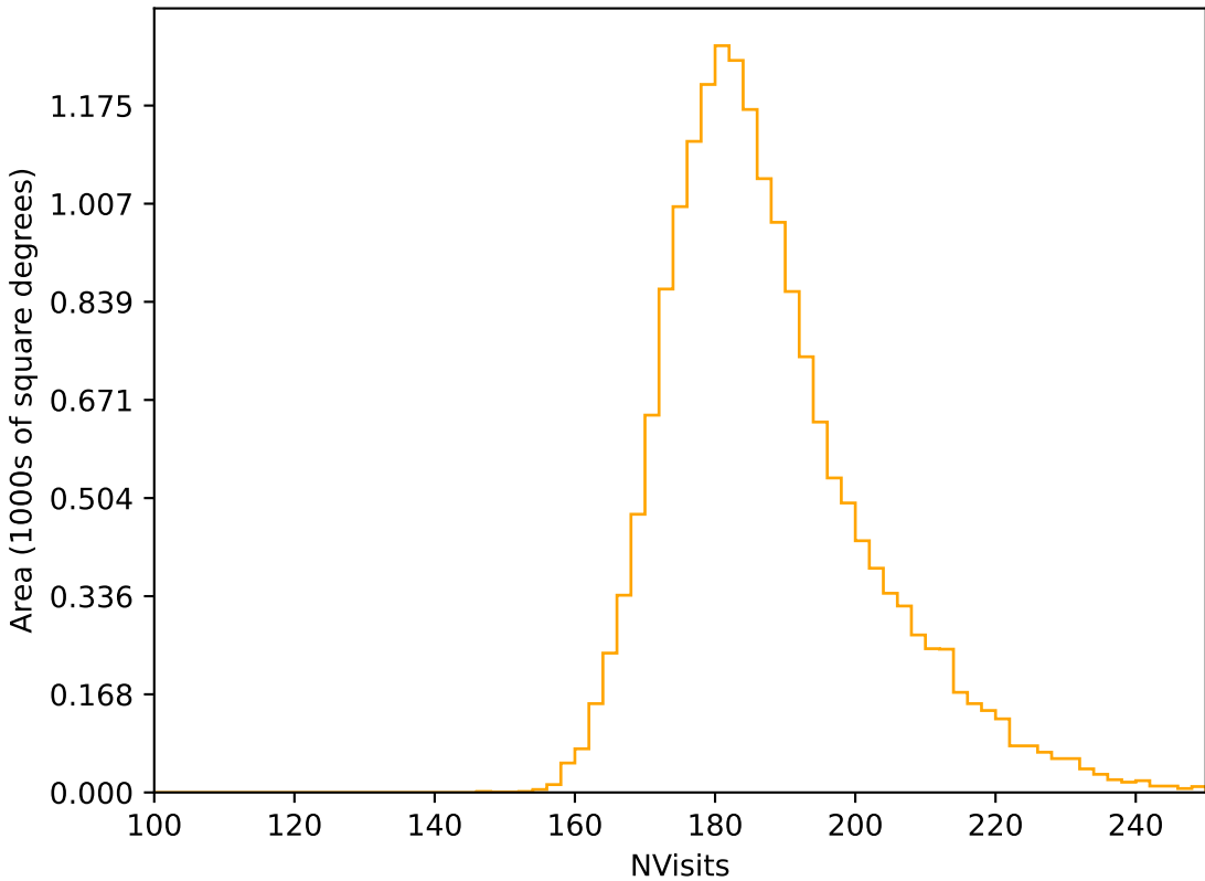
no_high_blob_v3.3_10yrs WFD r band: NVisits
