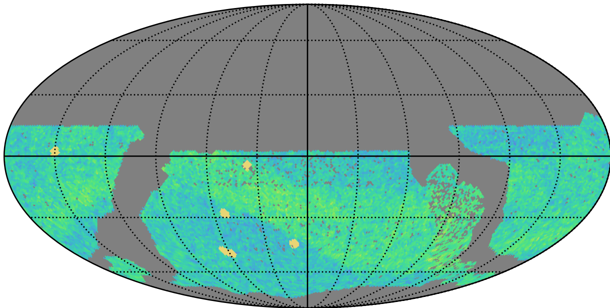
no_high_blob_v3.3_10yrs WFD i band: NVisits
