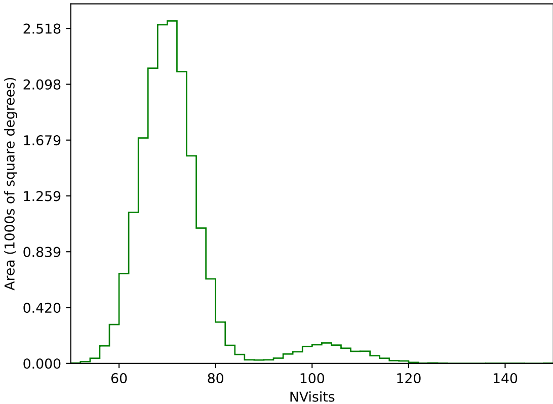
no_high_blob_v3.3_10yrs WFD g band: NVisits
