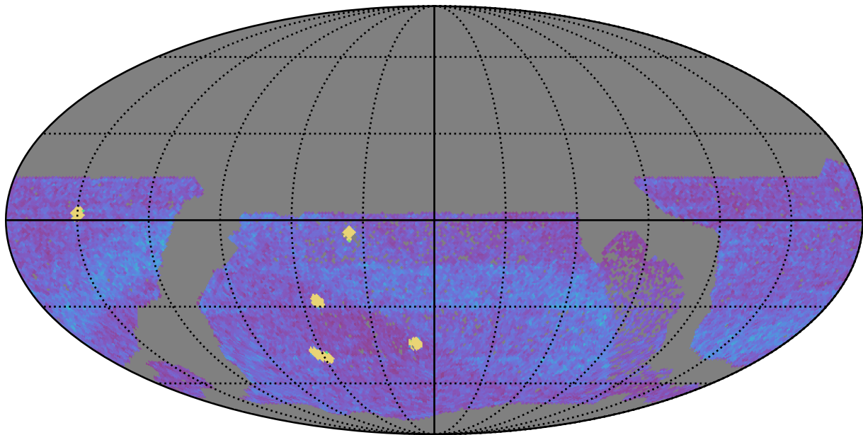
no_high_blob_v3.3_10yrs WFD all bands: NVisits
