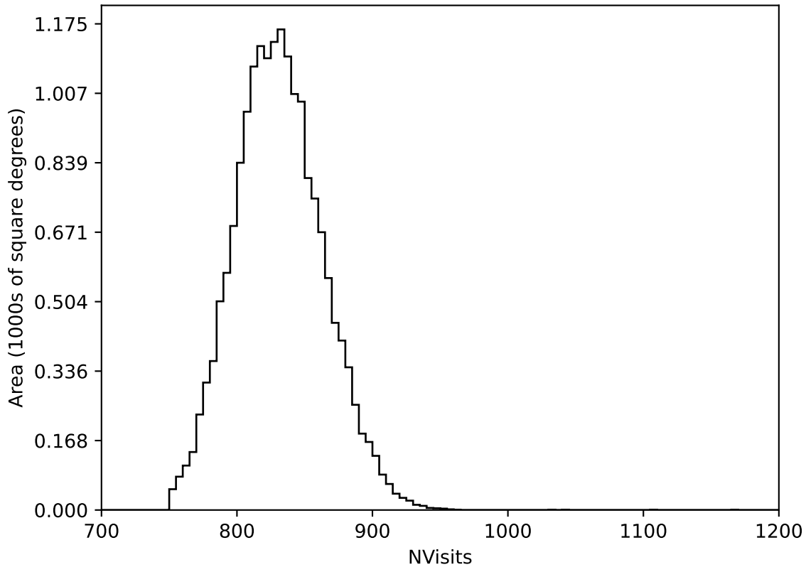
no_high_blob_v3.3_10yrs WFD all bands: NVisits
