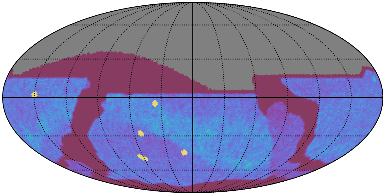
no_high_blob_v3.3_10yrs All sky z band: NVisits
