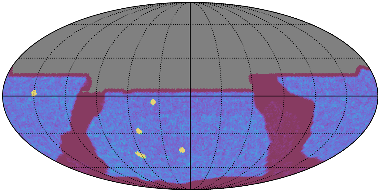
no_high_blob_v3.3_10yrs All sky y band: NVisits
