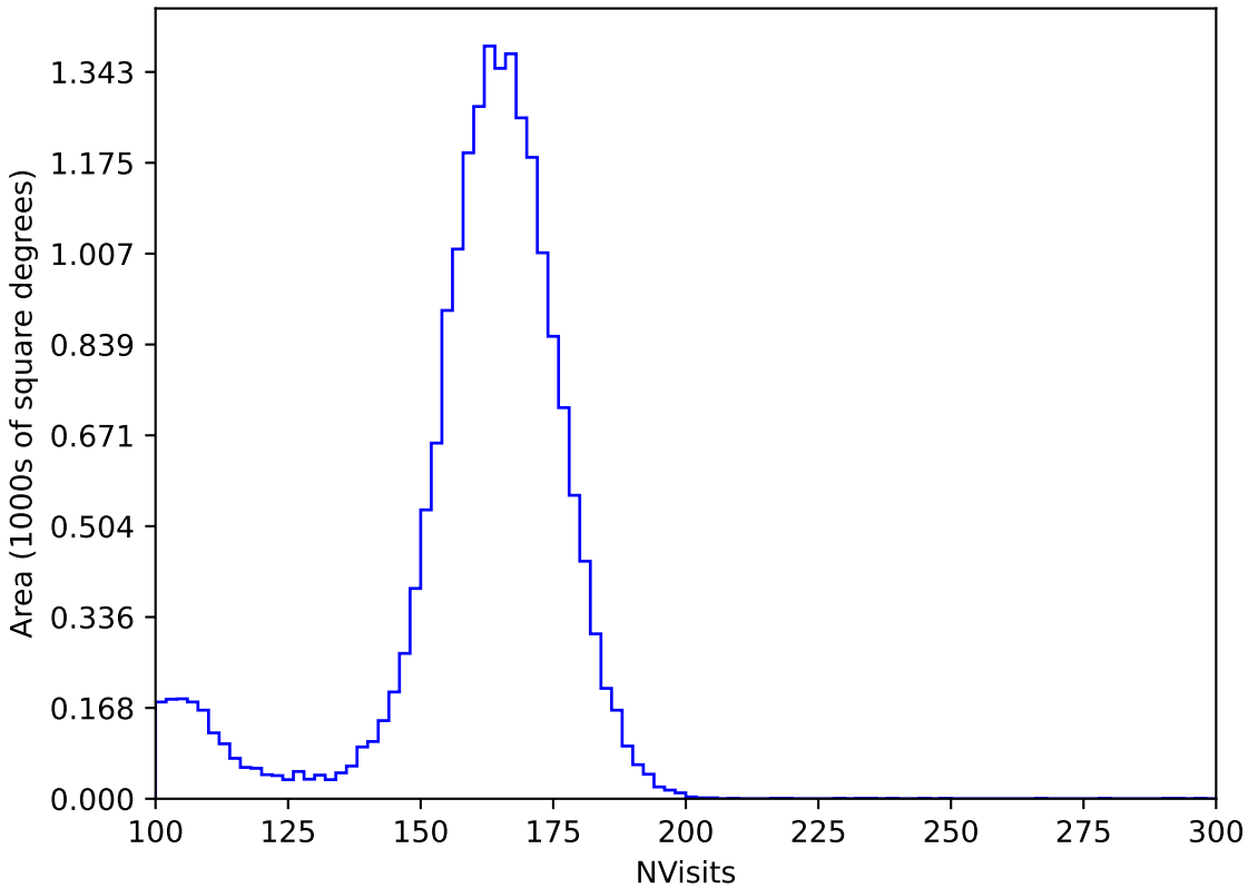
no_high_blob_v3.3_10yrs All sky y band: NVisits
