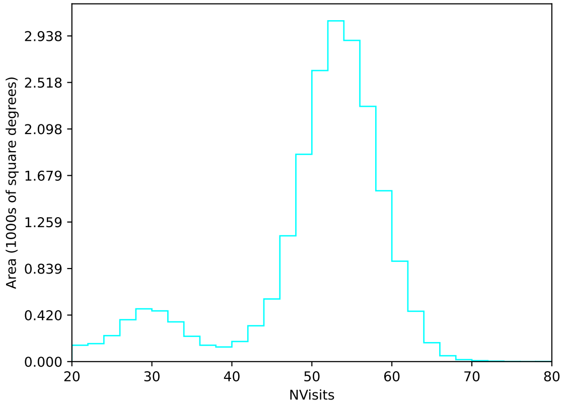
no_high_blob_v3.3_10yrs All sky u band: NVisits
