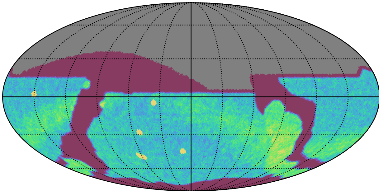
no_high_blob_v3.3_10yrs All sky r band: NVisits
