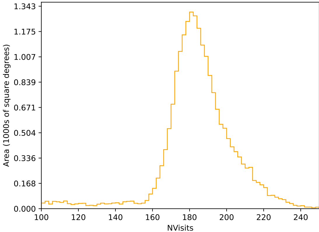
no_high_blob_v3.3_10yrs All sky r band: NVisits
