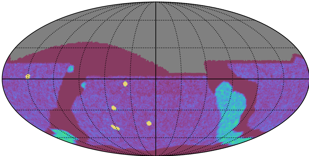
no_high_blob_v3.3_10yrs All sky g band: NVisits
