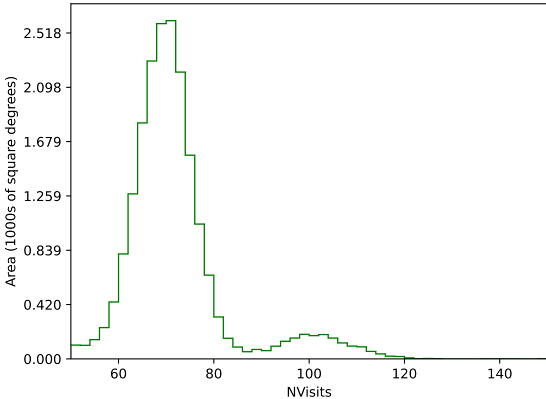
no_high_blob_v3.3_10yrs All sky g band: NVisits
