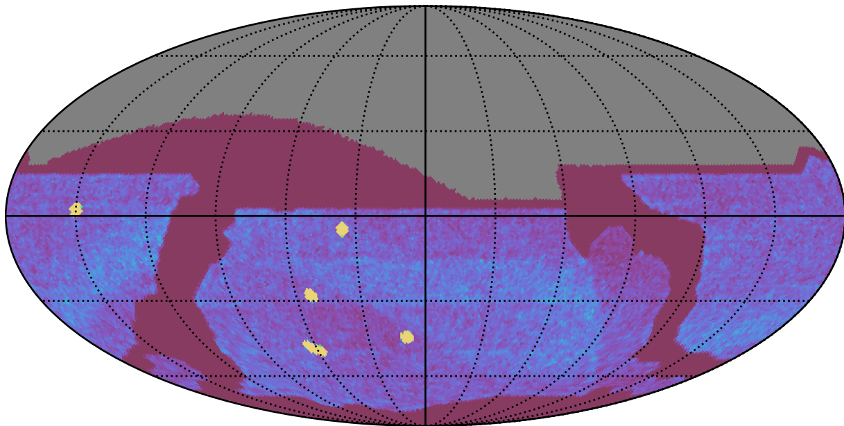
no_high_blob_v3.3_10yrs All sky all bands: NVisits
