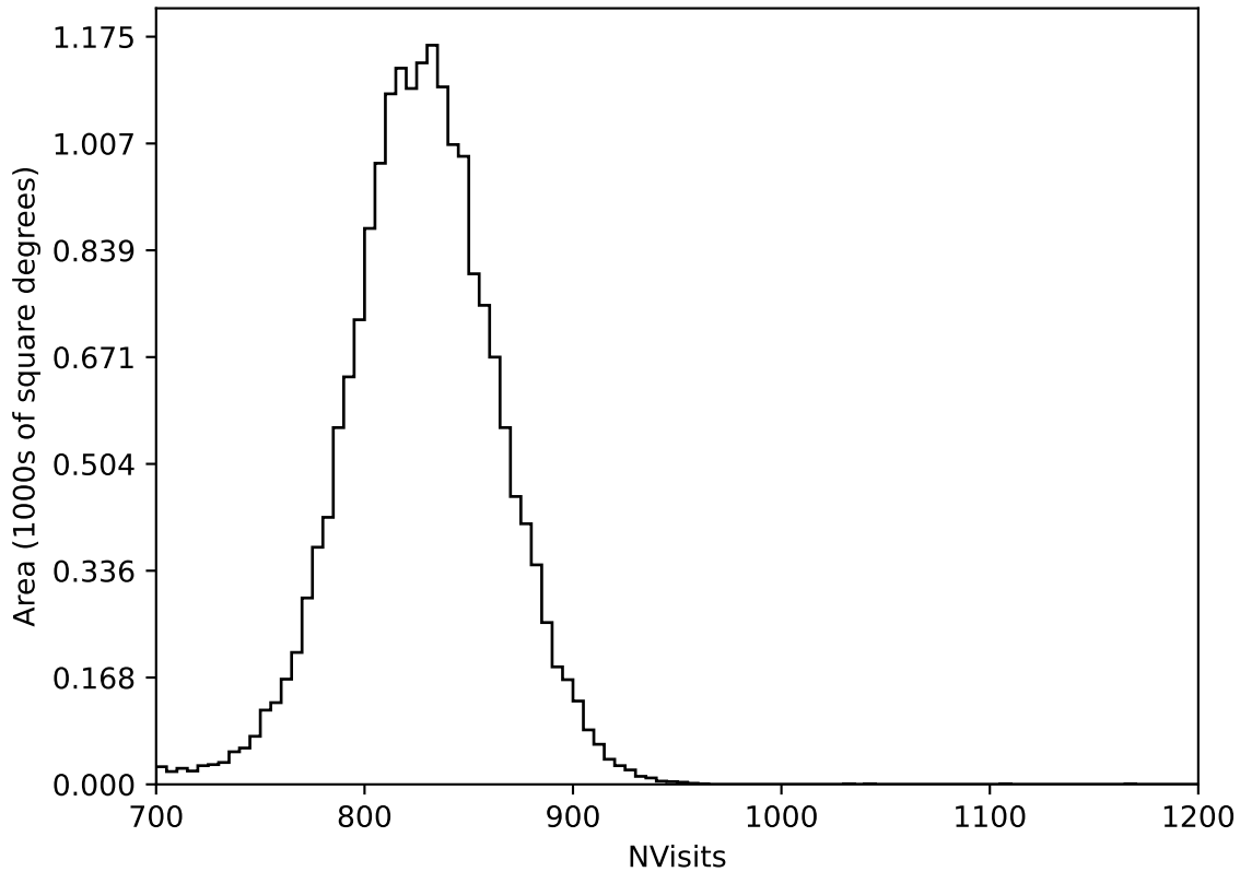
no_high_blob_v3.3_10yrs All sky all bands: NVisits
