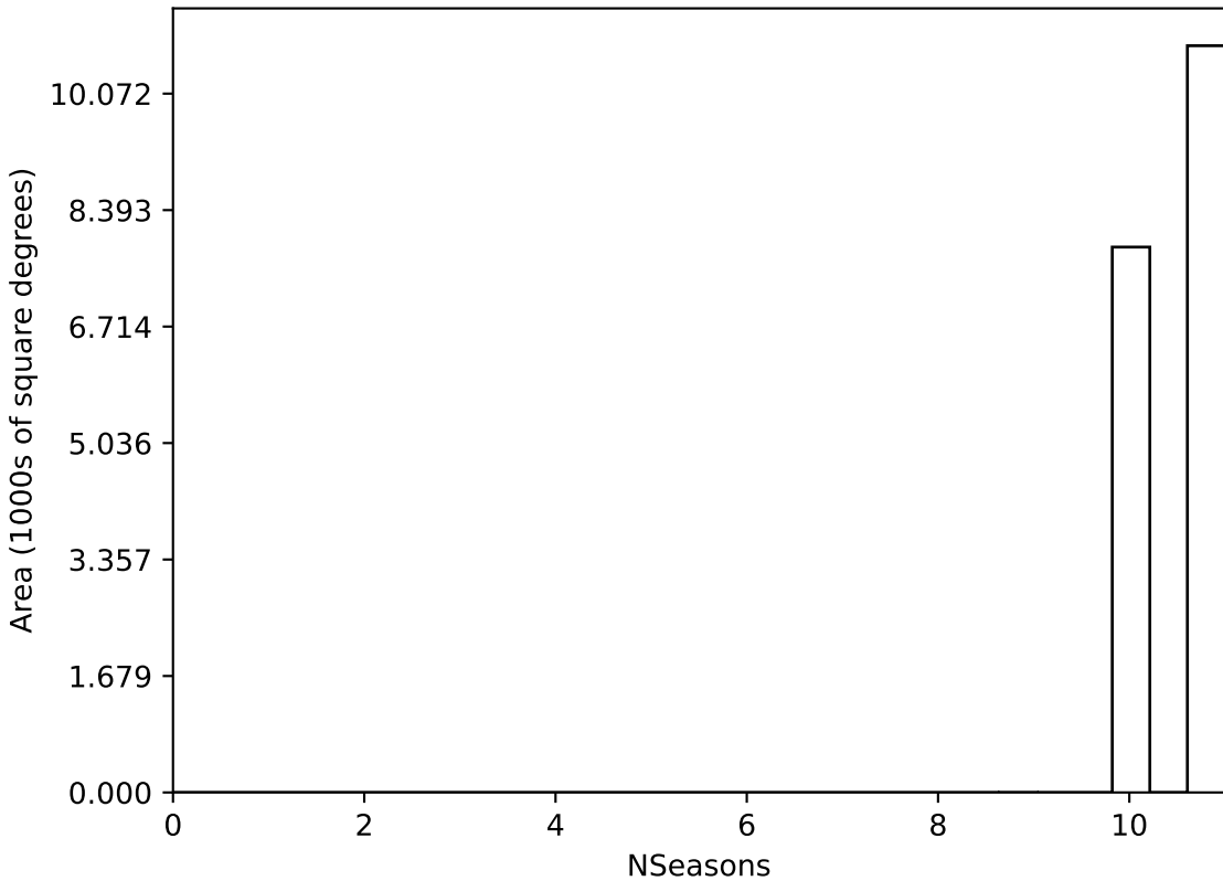
no_high_blob_v3.3_10yrs WFD all bands: NSeasons
