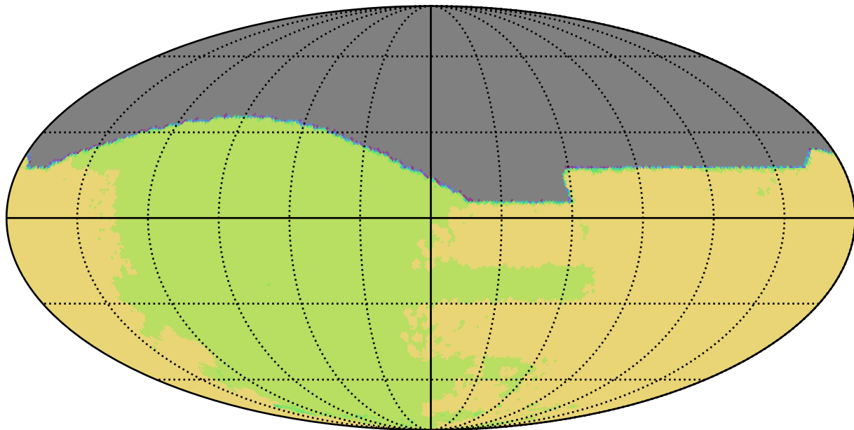
no_high_blob_v3.3_10yrs All sky all bands: NSeasons
