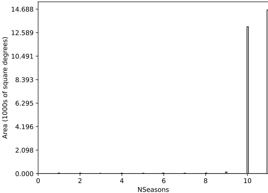
no_high_blob_v3.3_10yrs All sky all bands: NSeasons
