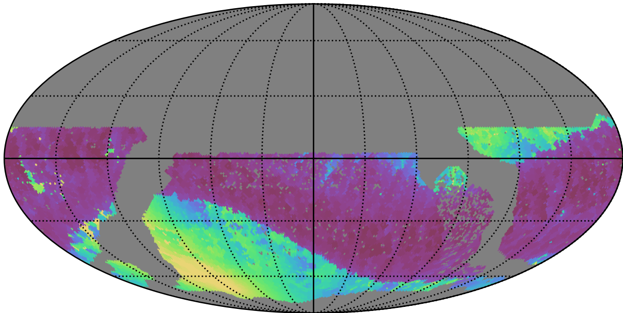
no_high_blob_v3.3_10yrs WFD z band: Min solarElong
