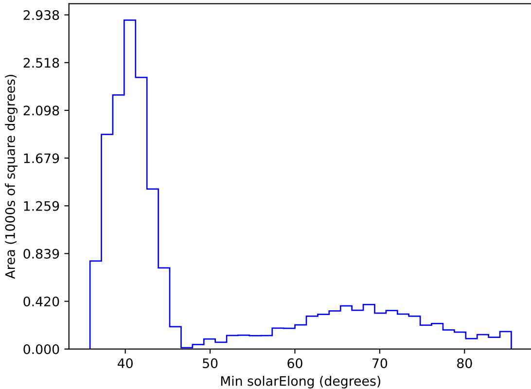
no_high_blob_v3.3_10yrs WFD z band: Min solarElong
