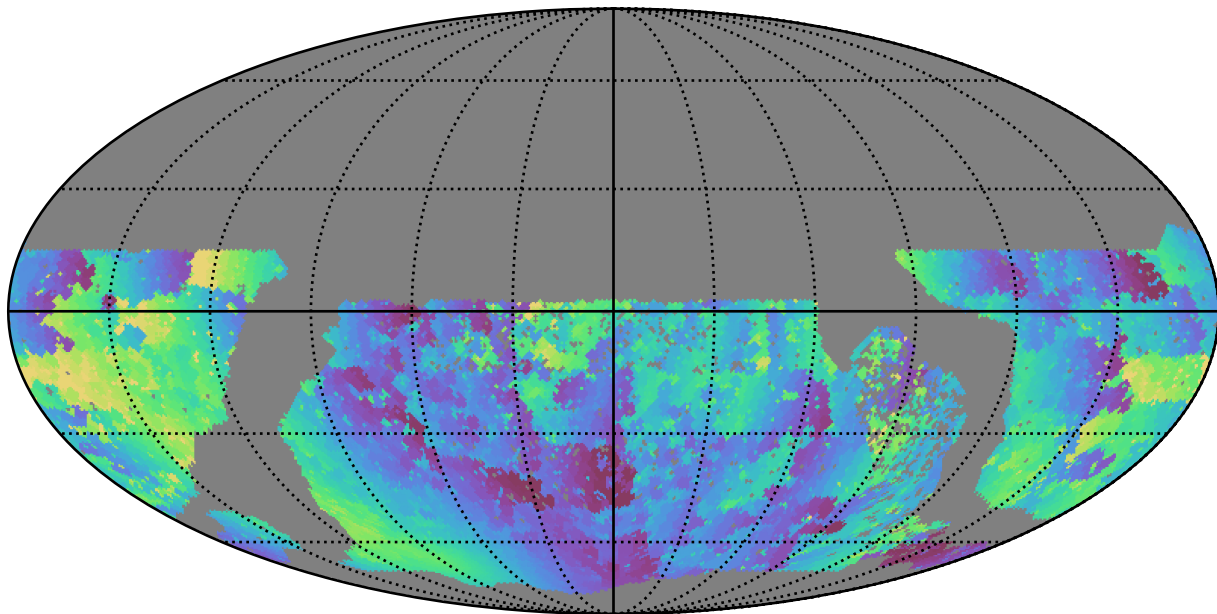
no_high_blob_v3.3_10yrs WFD u band: Min solarElong
