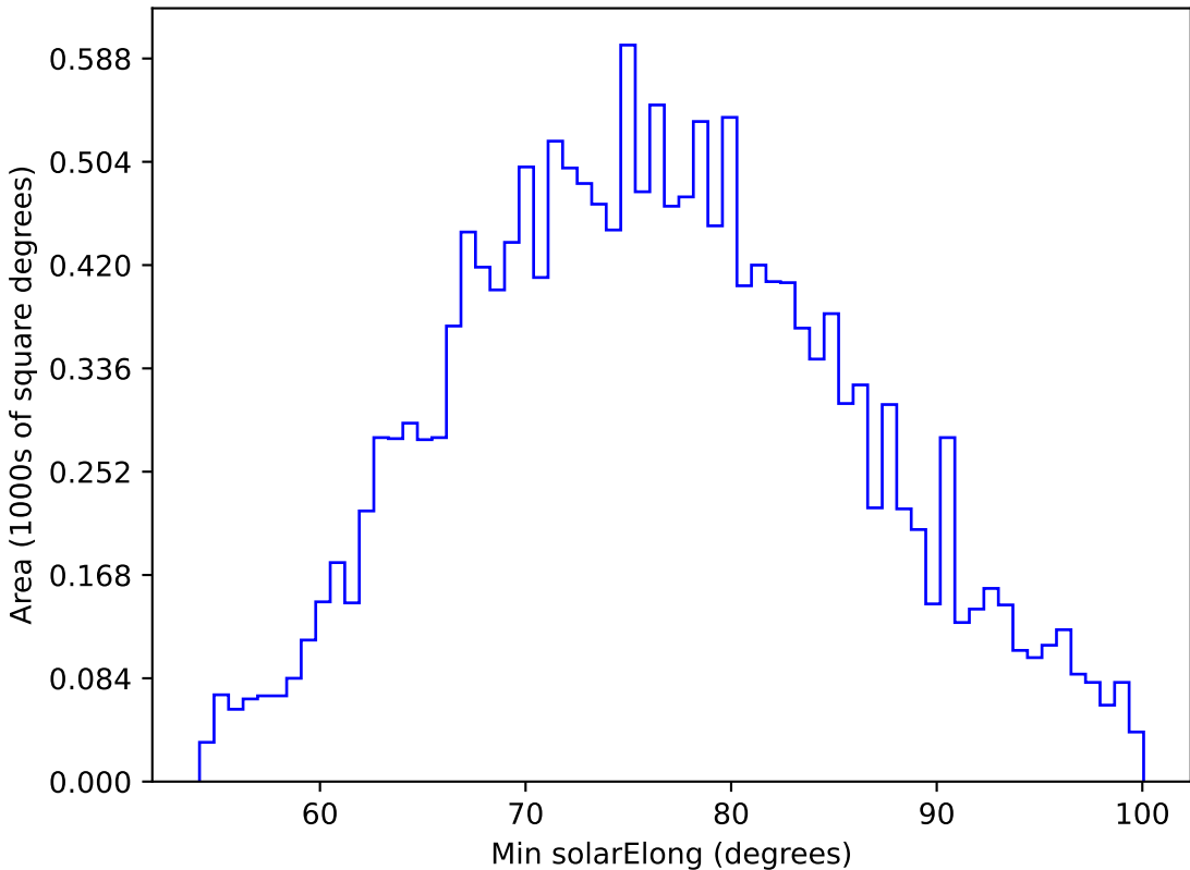
no_high_blob_v3.3_10yrs WFD u band: Min solarElong
