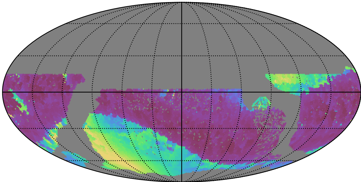
no_high_blob_v3.3_10yrs WFD i band: Min solarElong
