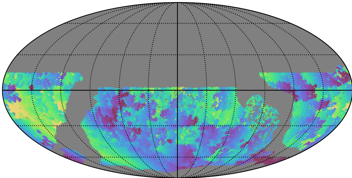
no_high_blob_v3.3_10yrs WFD g band: Min solarElong
