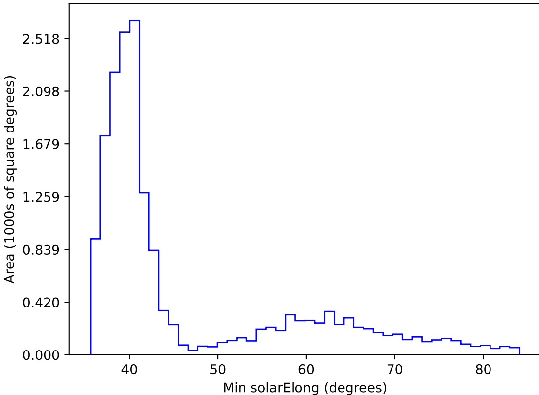
no_high_blob_v3.3_10yrs WFD all bands: Min solarElong
