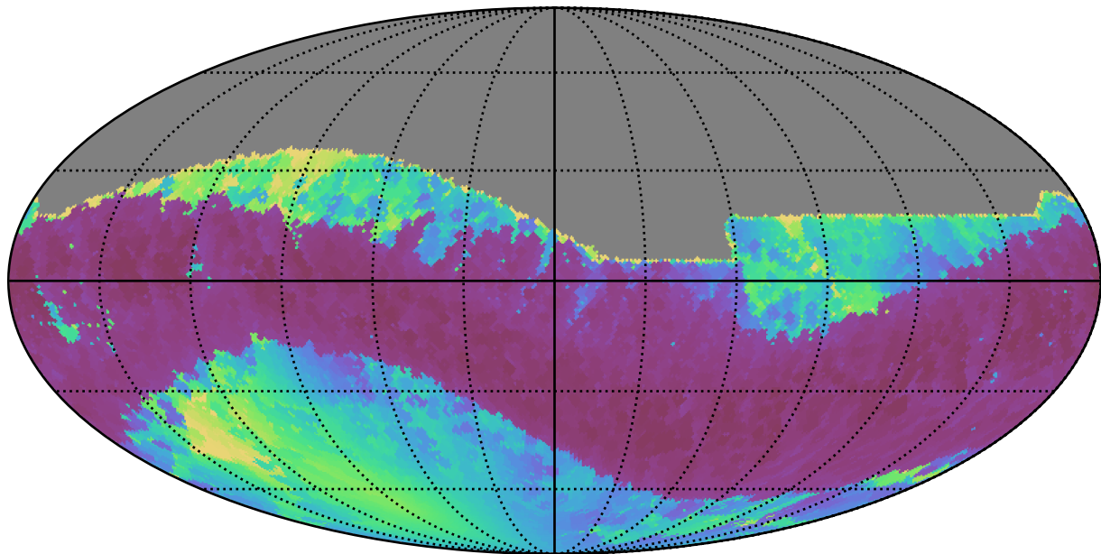
no_high_blob_v3.3_10yrs All sky z band: Min solarElong
