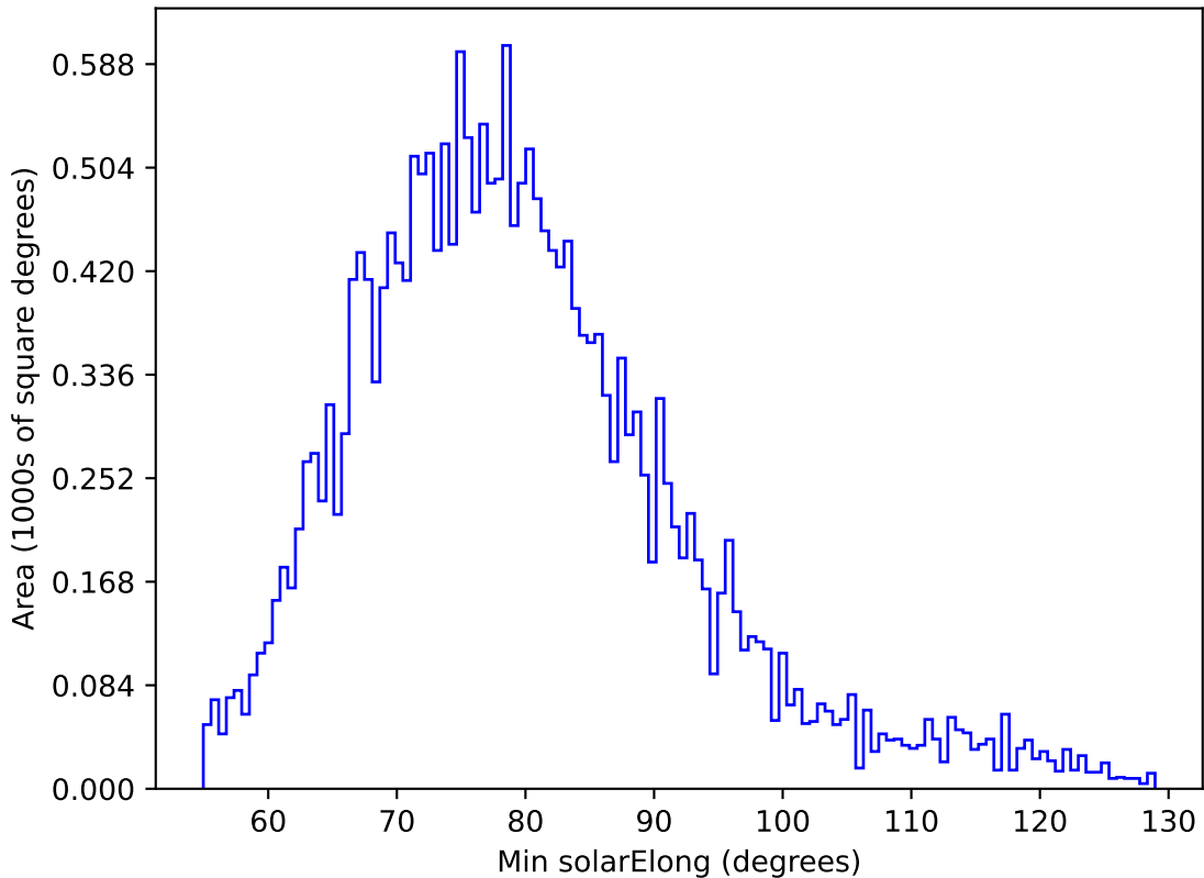
no_high_blob_v3.3_10yrs All sky u band: Min solarElong
