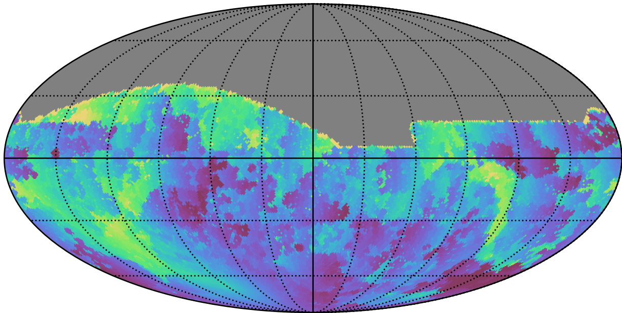
no_high_blob_v3.3_10yrs All sky g band: Min solarElong
