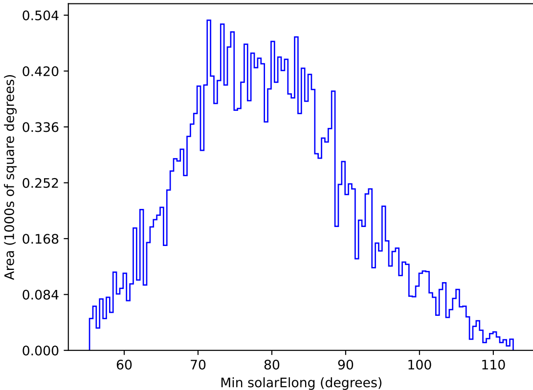
no_high_blob_v3.3_10yrs All sky g band: Min solarElong
