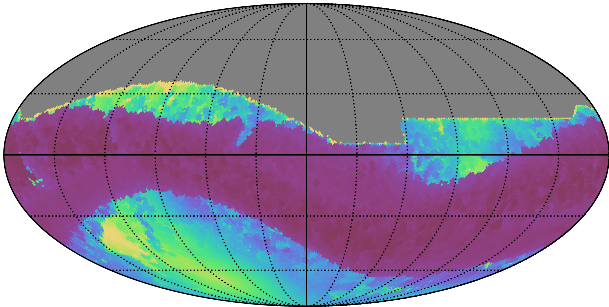
no_high_blob_v3.3_10yrs All sky all bands: Min solarElong
