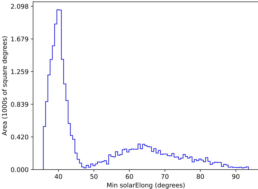
no_high_blob_v3.3_10yrs All sky all bands: Min solarElong
