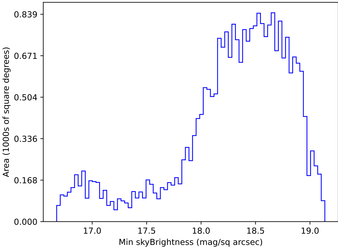
no_high_blob_v3.3_10yrs Yr 1 z band: Min skyBrightness
