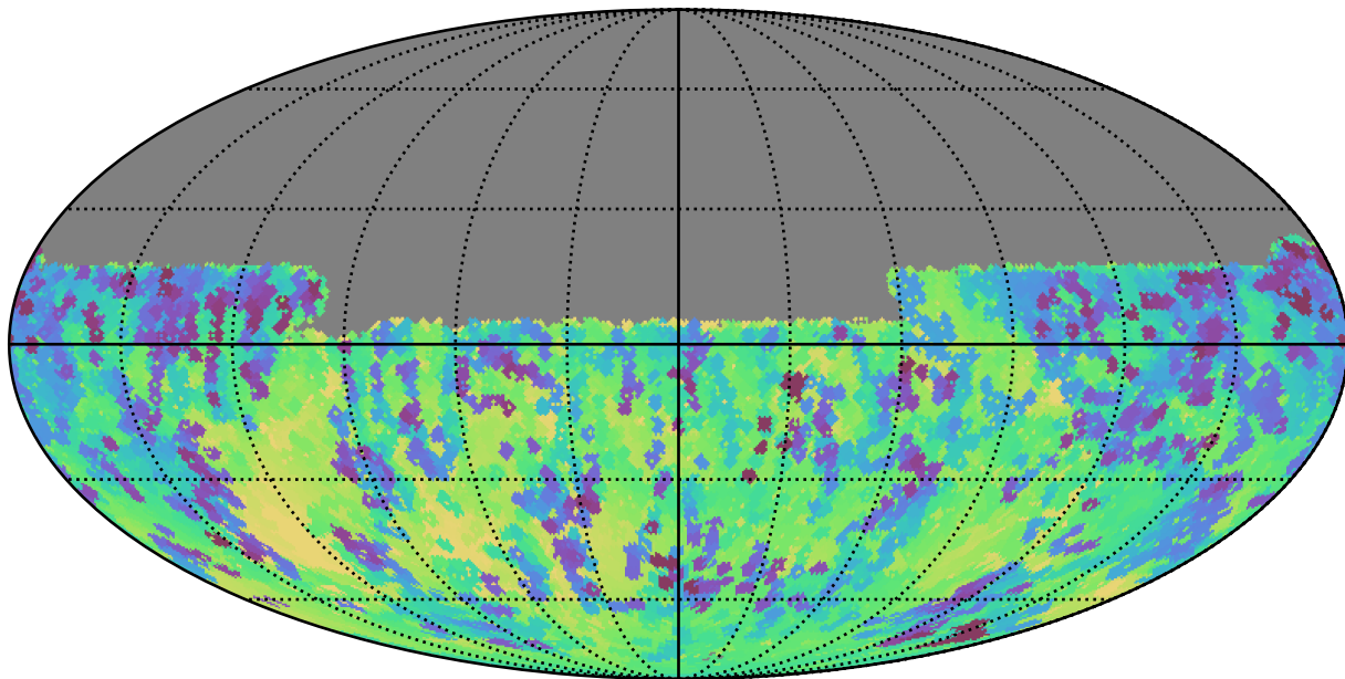
no_high_blob_v3.3_10yrs Yr 1 y band: Min skyBrightness
