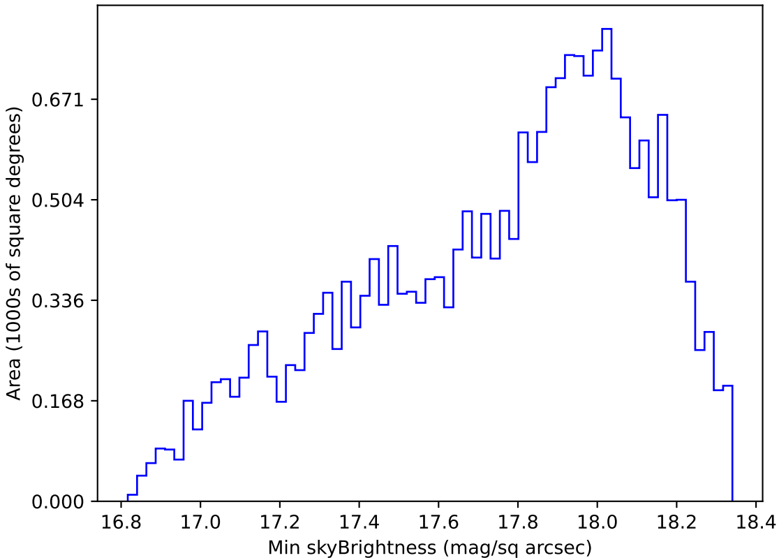
no_high_blob_v3.3_10yrs Yr 1 y band: Min skyBrightness
