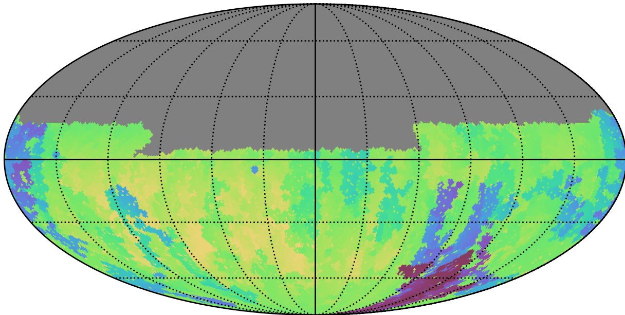
no_high_blob_v3.3_10yrs Yr 1 u band: Min skyBrightness
