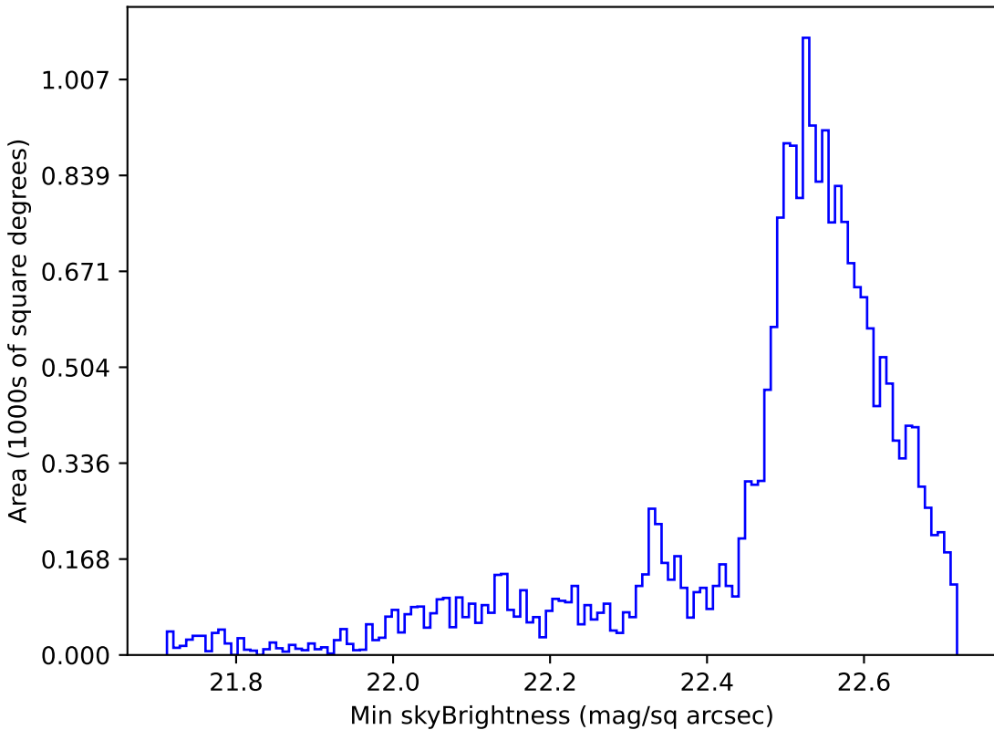
no_high_blob_v3.3_10yrs Yr 1 u band: Min skyBrightness
