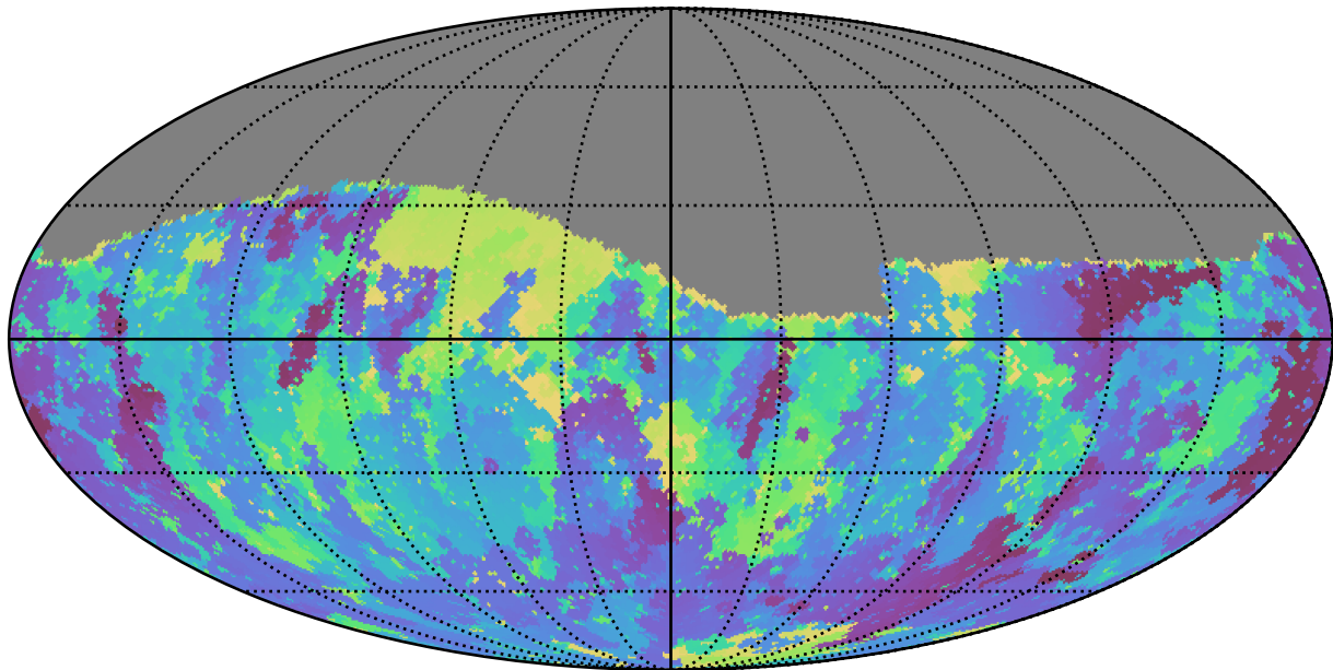
no_high_blob_v3.3_10yrs Yr 1 r band: Min skyBrightness
