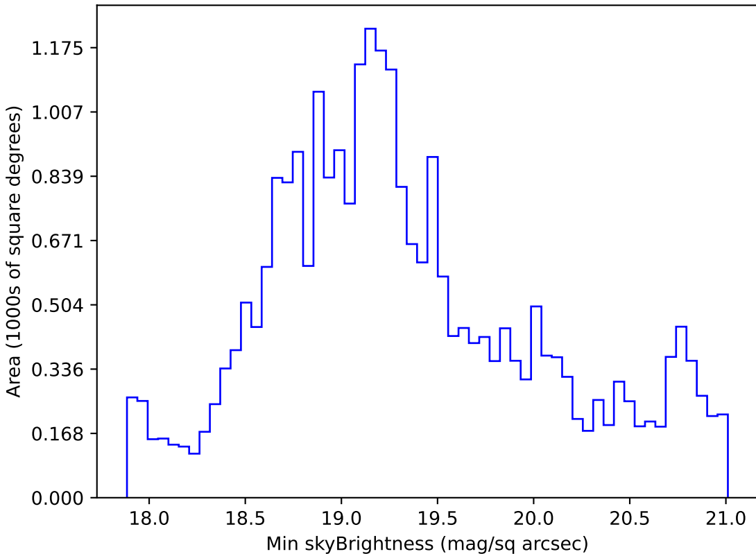
no_high_blob_v3.3_10yrs Yr 1 r band: Min skyBrightness
