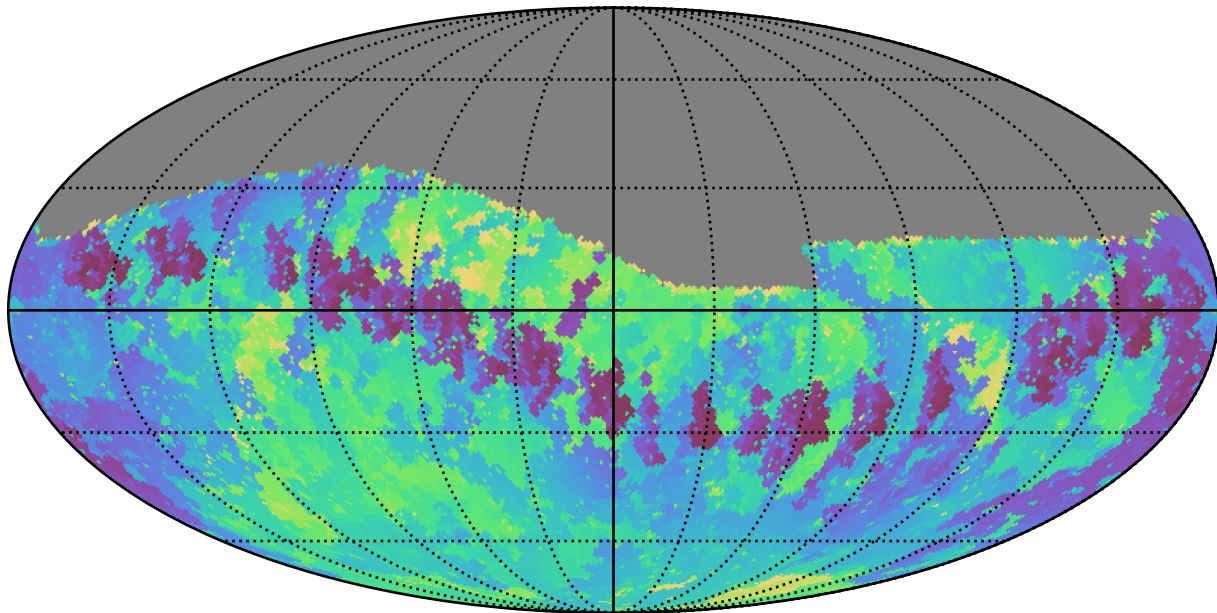
no_high_blob_v3.3_10yrs Yr 1 i band: Min skyBrightness
